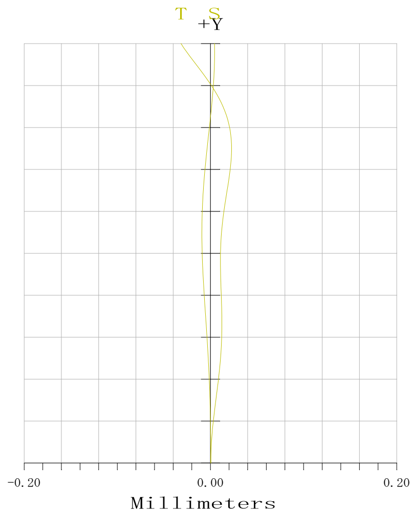
Field Curvature
