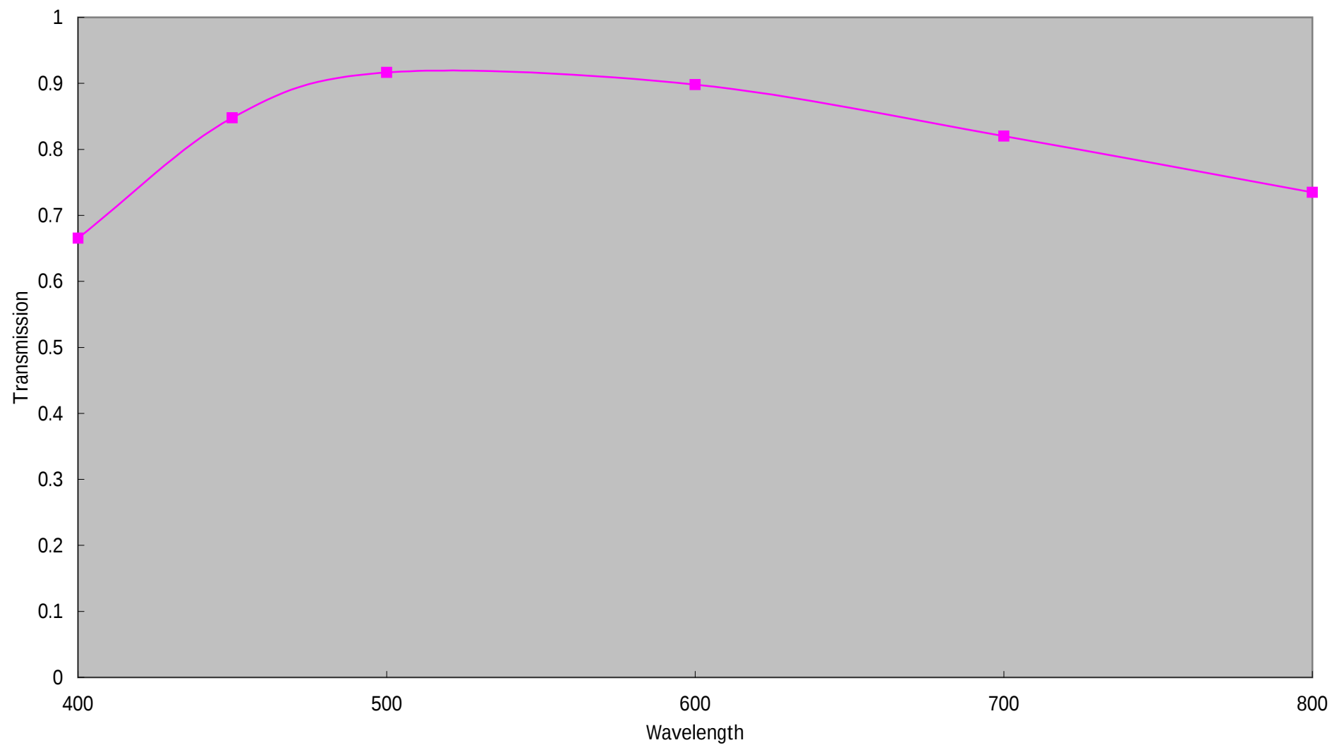
LM12NCL (604) Transmission
