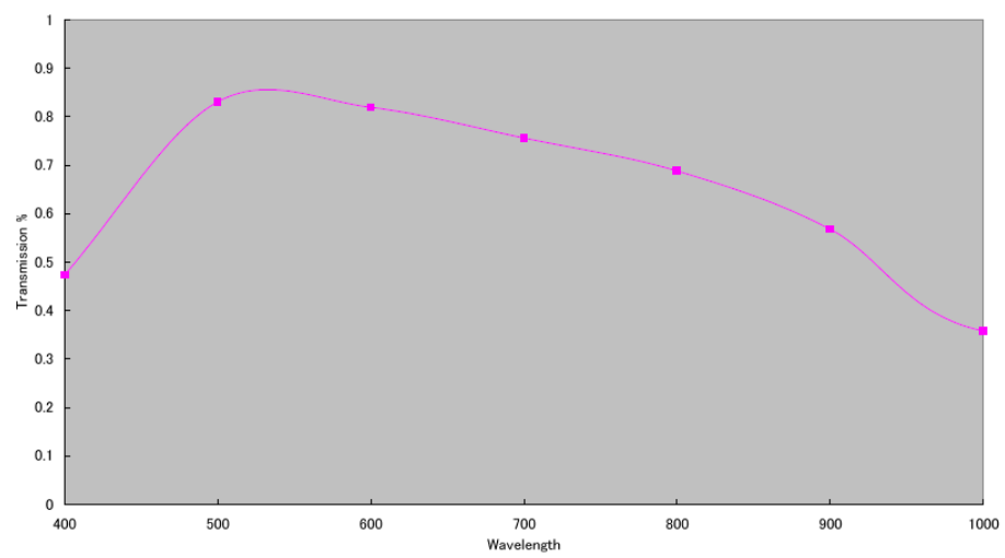
LMZ375 Transmission (standard coating )
