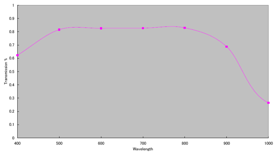
LMZ375 Transmission ( Broad Band Coating )
